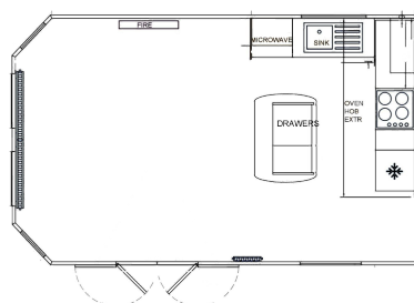
L SHAPED KITCHEN WITH ISLAND BAR FLOOR PLAN
