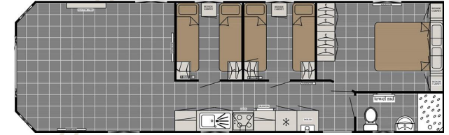
3 BED I SHAPED KITCHEN
